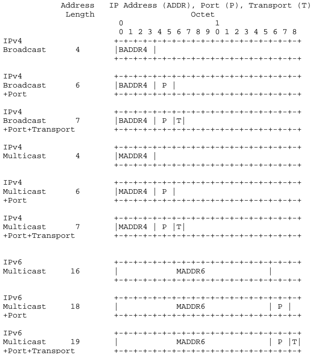
Figure 2: Encoding of broadcast/multicast native IP addresses
